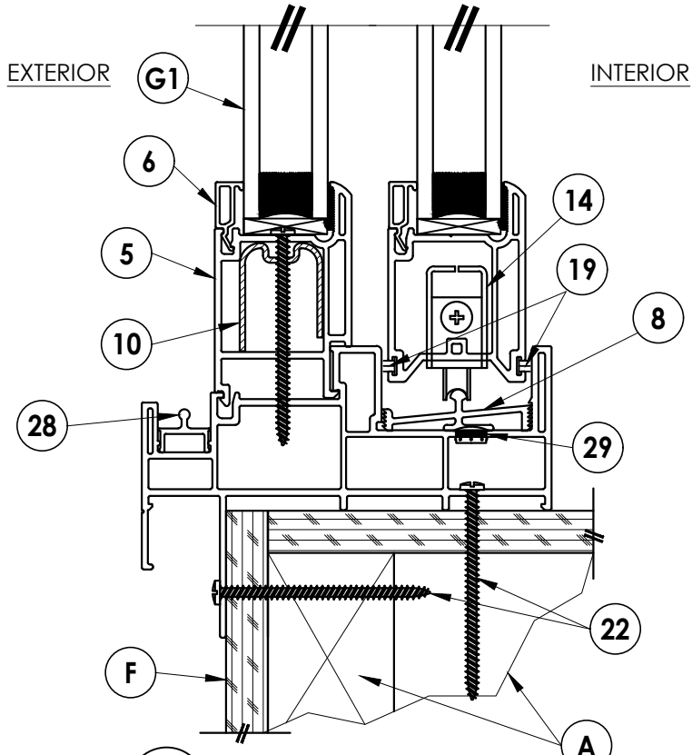
3 VERTICAL CROSS SECTION 3 Shown w/Stud framing option (On crawl space)
