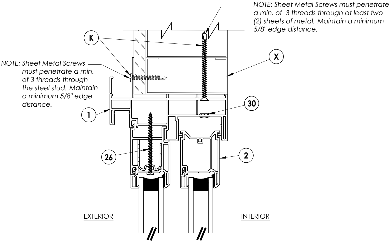
4 HORIZONTAL CROSS SECTION 3 Shown w/ Steel Stud framing option
